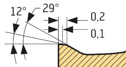
Corner radius
