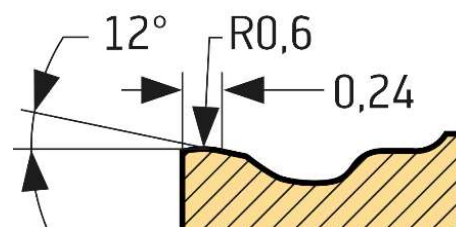
Main cutting edge
